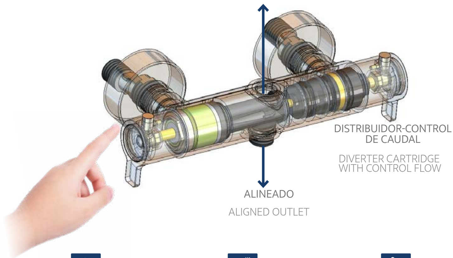
Cartucho termostático ref 1701 T Thermostatic cartridge
